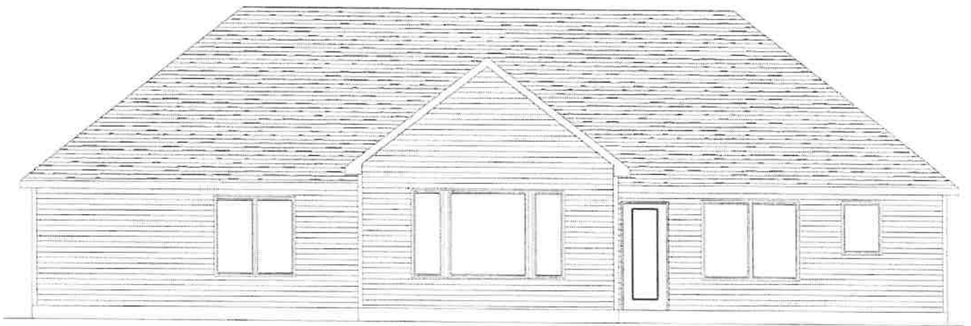
REAR ELEVATION
