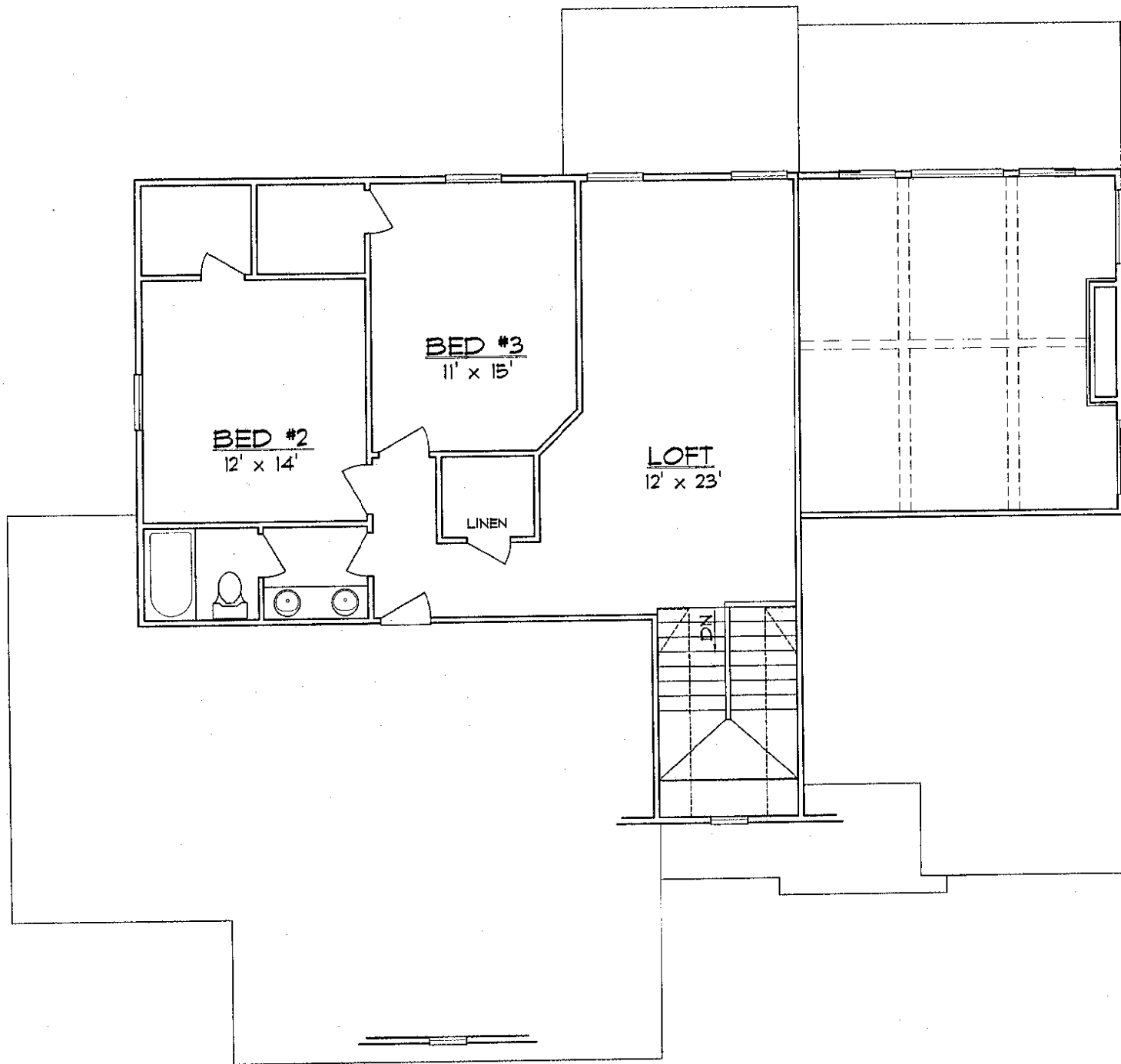
SECOND FLOOR
